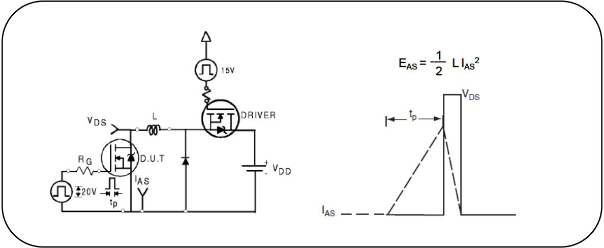
Fig. 10. Unclamped Inductive switching test circuit & waveform
