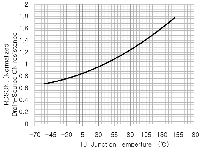
Fig. 5. On resistance variation vs. junction temperature
