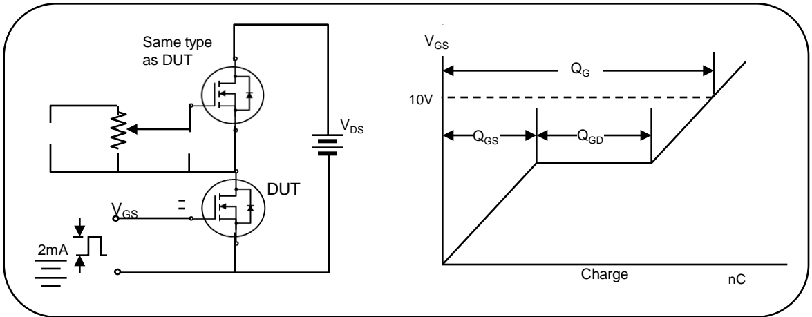
Fig. 8. Gate charge test circuit & waveform
