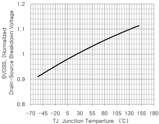
Fig 4. Breakdown Voltage Variation vs. Junction Temperature
